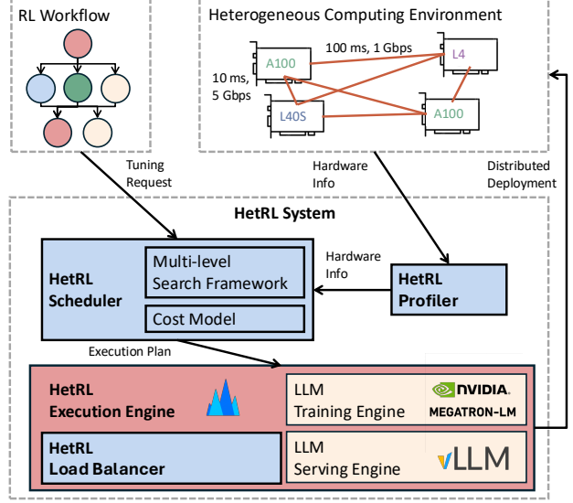
Figure 2. HetRL system overview.
