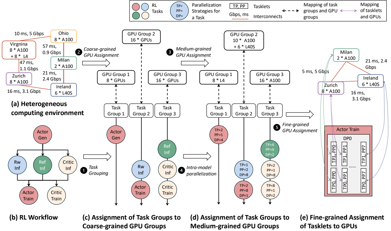
Figure 1. Given a heterogeneous computing environment (a) and an RL workflow (b), HetRL employs a multi-level search framework to progressively construct candidate execution plans through ① task grouping, ② coarse-grained GPU grouping, ③ medium-grained assignment of task groups to specific GPUs, ④ intra-model parallelization, and ⑤ fine-grained mapping of tasklets to GPUs. It enables efficient exploration of near-optimal solutions across sub-problems, while jointly optimizing task/model collocation, parallelization strategies, and device placement under heterogeneous compute and network resources.
