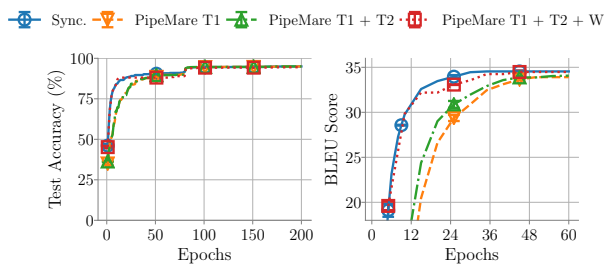
Figure 7. The impact of incrementally combining PipeMare techniques (T1, T2, and W) with ResNet50 on Cifar10 (left) and Transformer on IWSLT14 (right) with 107 and 93 pipeline stages respectively. Runs are stable across seeds indicated via the (negligible) error bars in each plot.
