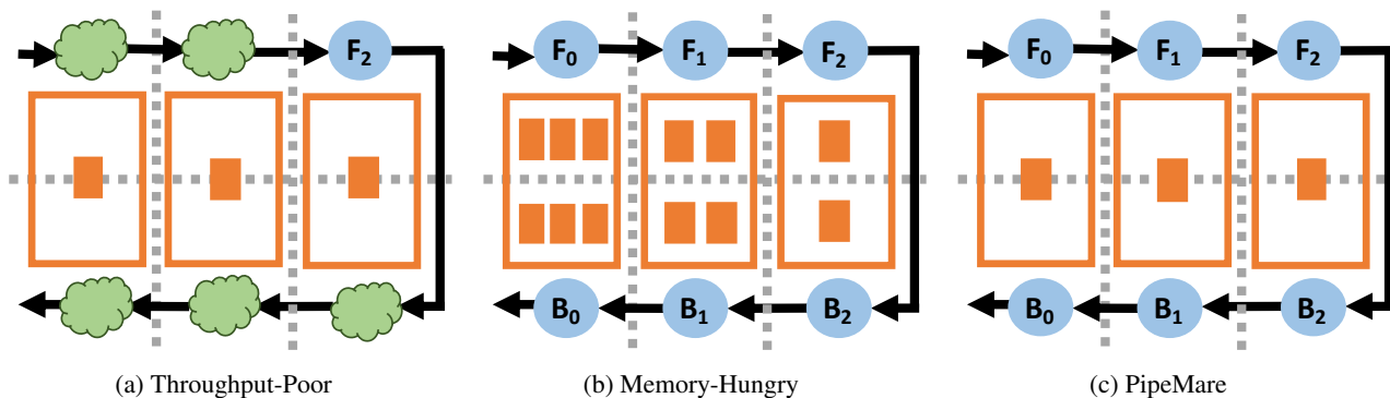
Figure 1. Different extremes of pipelining modes. Orange squares represent model weight memory, blue circles represent active pipeline compute, green clouds represent pipeline bubbles, and dashed gray lines separate pipeline stages. PipeMare fully utilizes compute while minimizing weight memory footprint.
