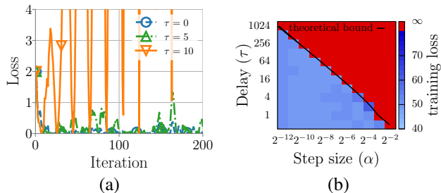
Figure 5. (a) Increasing \tau can cause the quadratic model to diverge even when \alpha remains fixed. (b) Evaluation of pipeline-parallel SGD for linear regression on the cpusmall dataset running for T = 10^6 iterations. The heatmap reports losses as a function of the step size \alpha and the delay \tau ; red denotes divergence to \infty . The black curve shows the upper bound from Lemma 1 using the largest curvature of the objective in place of \lambda .
