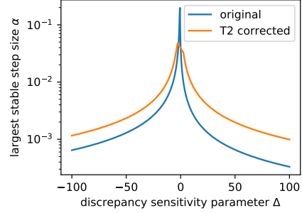
Figure 10. Plot of the largest step size \alpha for which all the eigenvalues of the companion matrix lie within the unit disk for various values of the discrepancy sensitivity parameter \Delta , comparing the original quadratic model with the T2 discrepancy-corrected model. This figure was generated for \tau_{\text{fwd}} = 40 and \tau_{\text{bkwd}} = 10 .
