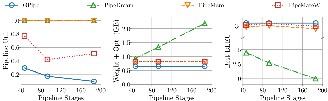
Figure 3. The impact of the number of pipeline stages on pipeline utilization, weight and optimizer memory, and final model quality across different pipeline parallel training methods on a 12-layer Transformer model performing machine translation on the IWSLT14 dataset. Similar to image classification task, GPipe and PipeDream suffer hardware costs proportional to the number of pipeline stages. Without these costs, PipeMare can achieve a final model quality close to the best technique and with a few warm-up epochs, PipeMareW (with warmup epochs, see Section 4) can further close the gap. The target BLEU score chosen to evaluate the amortized pipeline utilization of PipeMareW is 33.9.
