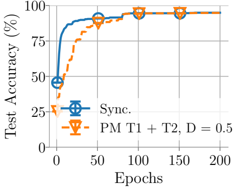
Figure 12. We observe ResNet 152 on CIFAR20 diverges when only using learning rate rescheduling (T1). Discrepancy correction is necessary to prevent divergence for ResNet 152 on CIFAR10; we observe PipeMare with discrepancy correction (T1 + T2) attains matching performance to GPipe synchronous training.
