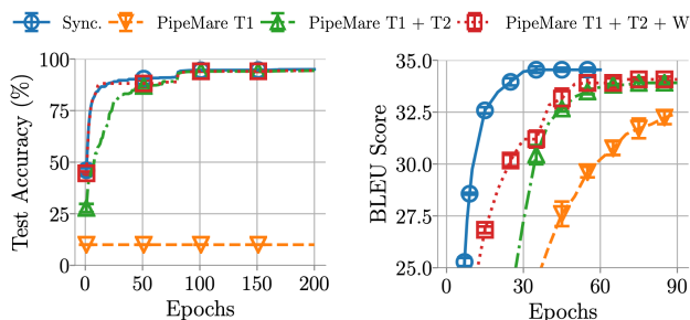
Figure 8. The impact of incrementally combining PipeMare techniques (T1, T2, and W) with ResNet50 on Cifar10 (left) and Transformer on IWSLT14 (right) with 214 and 186 pipeline stages respectively. This doubles the number of pipeline stages as compared to Figure 7. It explores the limits of our approach at an even finer granularity of pipeline parallelism.
