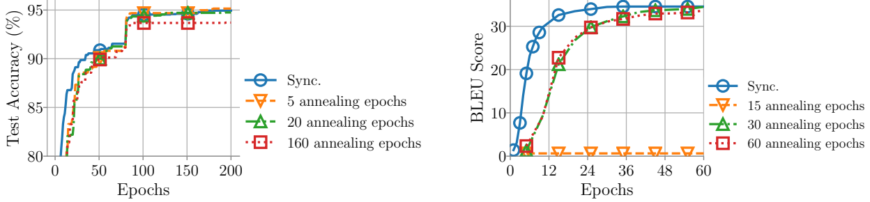
Figure 13. Sensitivity of model accuracy to the number of annealing epochs. We observe that choosing the number of annealing epochs can be important to achieving model accuracy matching synchronous training.
