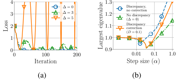
Figure 6. (a) Increasing \Delta , the gradient sensitivity to delay discrepancy, can cause the quadratic model to diverge even when \alpha and \tau remain fixed, using \tau_{\text{fwd}} = 10 , \tau_{\text{bkwd}} = 6 , and \lambda = 1 . (b) Effect of discrepancy correction on the quadratic model. Forward-backward delay discrepancy (blue) increases the largest magnitude eigenvalue of the companion matrix with \Delta = 5 , and \tau , \lambda same as in (a). Discrepancy correction with D = 0.1 (orange) reduces the largest magnitude eigenvalue; this eigenvalue is closer to that attained without delay discrepancy (green).
