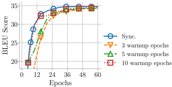
Figure 15. Sensitivity of model accuracy to the number of synchronous warmup epochs on IWSLT. We observe a tradeoff in using warmup epochs: a large number of warmup epochs can harm the throughput but converges to a good model accuracy in fewer epochs.
