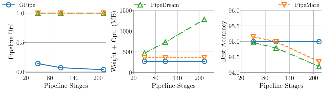
Figure 2. The impact of the number of pipeline stages on pipeline utilization, weight memory, and final model quality across different pipeline parallel training methods on a ResNet50 for image classification with the CIFAR10 dataset. Unlike PipeMare, GPipe and PipeDream suffer hardware costs (either throughput or the sum of weight and optimizer memory) proportional to the number of pipeline stages. Still, PipeMare achieves a final model quality competitive with the best technique.
