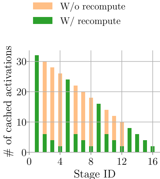
Figure 9. Activation memory footprint of PipeMare recompute in each pipeline stage. In this plot, we demonstrate the # of activations at each stage using an example with 16 stages equally split into 4 segments. The green bars in the plot stands for the memory consumption of each stage in terms of the number of microbatch activations copies in PipeMare with PipeMare recompute. The orange bars stands for the additional memory required when recompute is not used.
