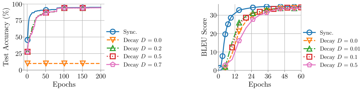
Figure 14. Sensitivity of model accuracy to the decay D for discrepancy correction. We notice that the decay value can have an impact on the convergence speed. For example, it requires a decay smaller than 0.5 to converge faster than without discrepancy correction while 0.5 can demonstrate test accuracy matching that attained by synchronous training.
