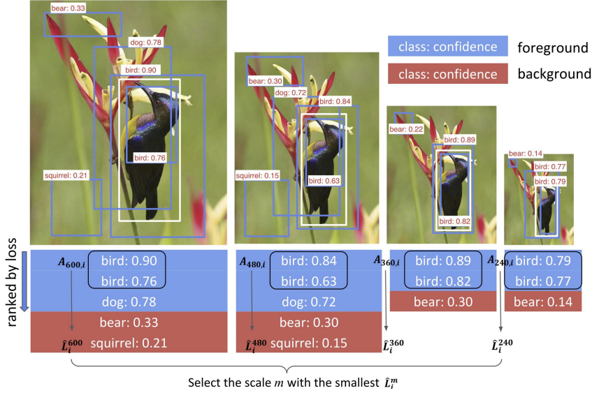
Figure 3. Optimal scale determination. First, the same number of predicted foregrounds from four scales are selected as A_{m,i} . Then, the scale with the lowest loss L_i^m is selected as the optimal scale.
